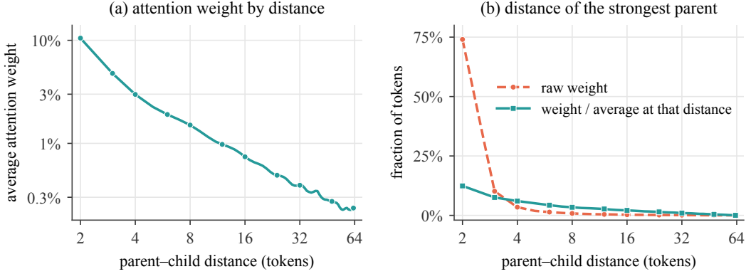
Figure 2: Attention of Qwen3-8B-Base on 1,400 FineMath-4+ documents . (a) Average attention weight on an earlier token j by parent-child distance i - j . (b) Distance of each token’s strongest parent when parents are ranked by the raw weight or by the weight divided by the average weight at that distance.
