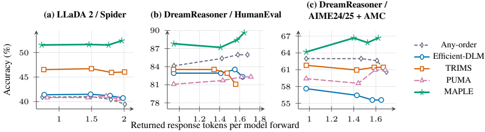
Figure 1: Accuracy-parallelism trade-offs from confidence-threshold sweeps of the same final checkpoints as Table 1 over \tau \in \{0.95, 0.97, 0.99, 1.00\} . The rightmost point of each curve is \tau = 0.95 , the recommended setting for LLaDA 2 and DreamReasoner. Parallelism is returned response tokens per model forward.
