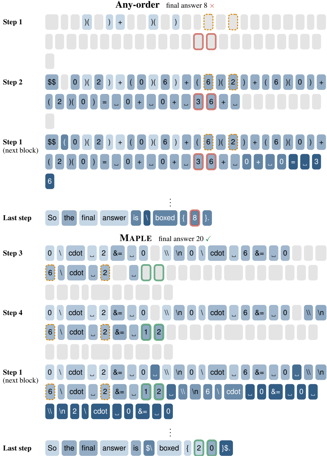
Figure 5: OlympiadBench. Problem: compute the area of pentagon TNYWR with T = (0, 0) , N = (2, 0) , Y = (6, 6) , W = (2, 6) , and R = (0, 2) (answer 20). Shown: the products y_i x_{i+1} of the shoelace formula (and, for the any-order model, their sum), then the final answer. Legend as in Figure 3.
