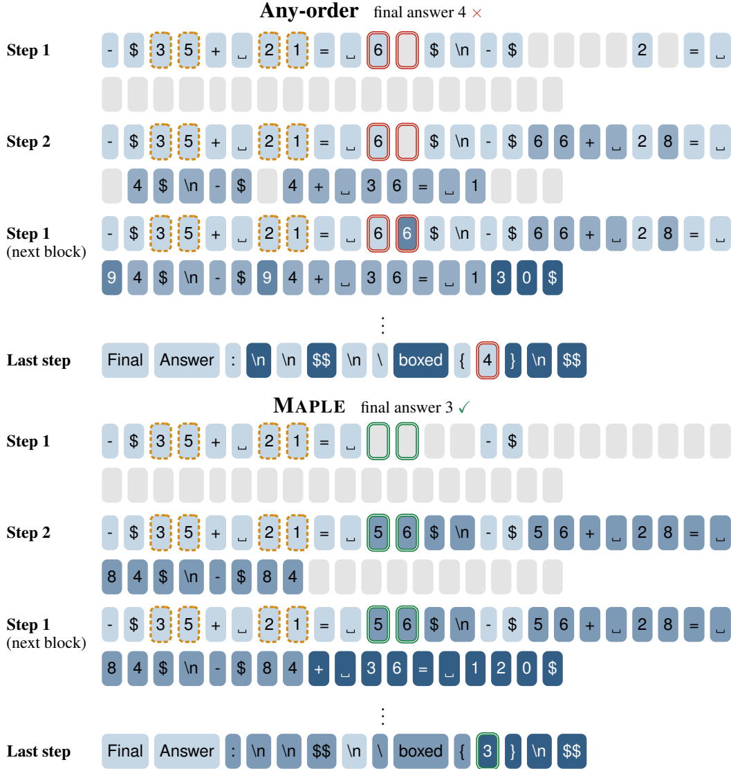
Figure 3: MATH500. Problem: find n with 0 \leq n < 9 and 1 + 12 + 123 + \dots + 12345678 \equiv n \pmod{9} (answer 3). Shown: the running sums of the digit sums at the decoding steps given on the left, then the final answer. Steps are counted within the 64-token block being decoded, and rows need not be consecutive steps. Gray : masked; shade: step of commitment, from light (earlier) to dark (later); solid border : tokens that decide the answer; dashed border : tokens they are computed from.
